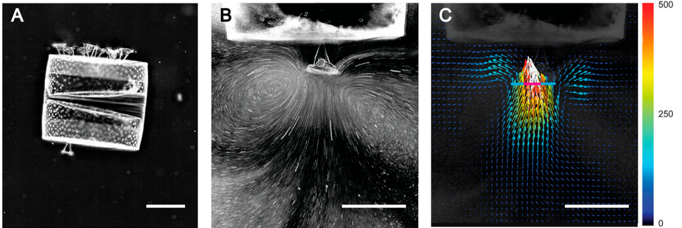
Fig. 1. Diatom-ciliate association: (A) diatom C. walesii and its epibiont P. coscinodisci . Scale bars represent 100 microns in length. (B) Flow around a single ciliate directed toward the diatom cell surface. (C) Velocity field for the same diatom-ciliate pair with a blue line indicating the transect line used for measurement of flow field velocities. The magenta segment represents the microcurrent component that directly intercepts the ciliary crown.
