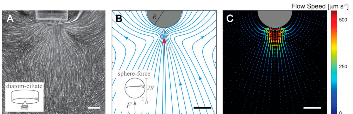
Fig. 2. Diatom-ciliate model: (A) Streamlines of particle paths generated by the flow field of a three-member cluster of the ciliate P. coscinodisci attached to the diatom C. walesii . (B) Streamlines produced by the diatom-ciliate model consisting of a sphere of radius R and a regularized Stokeslet of dimensionless strength F = 10 and regularization parameter r = 0.4 R located at a distance h = 0.5 R from the sphere's south pole and pointing toward the sphere's center. (C) Velocity field for the same diatom-ciliate model. Scale bars represent 100 microns in length.
